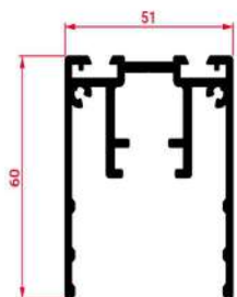
PERFIL COMPENSADOR SUPERIOR | PROFIL COMPENSATEUR SUPERIEUR | UPPER EXPANSION JOINTS FRAME
